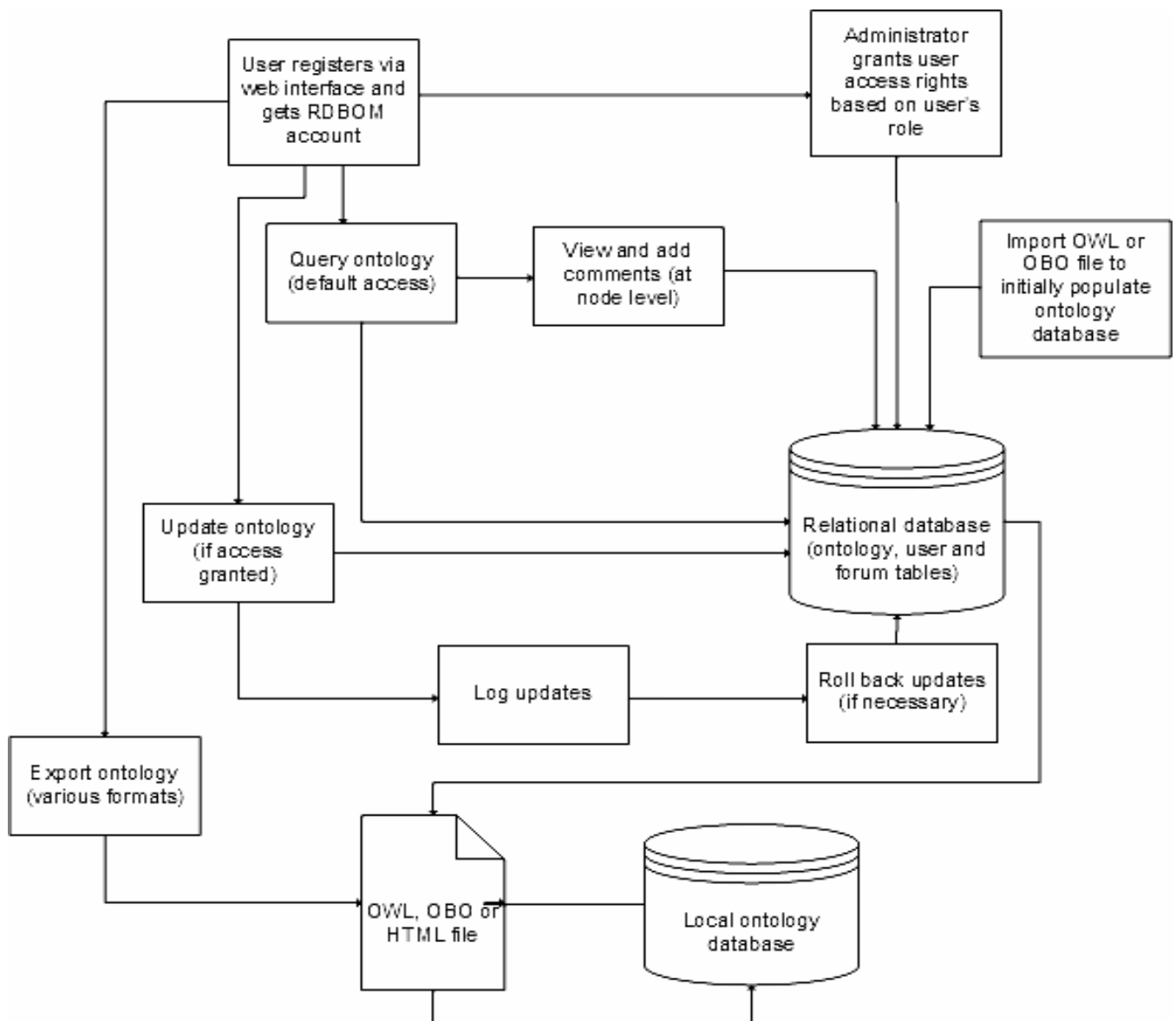
Fig. 4. RDBOM collaborative workflow
